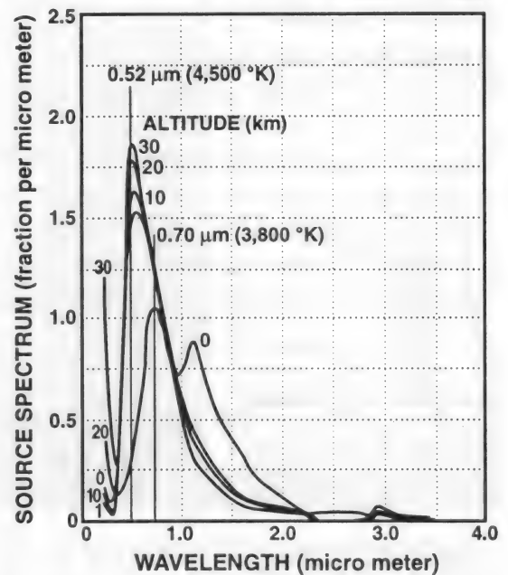
Figure 6.21. Effect of Altitude on Spectral Distribution for a 1-MT Burst.
