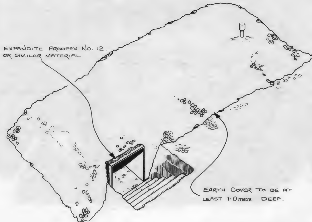
Fig. 91 Earth cover
