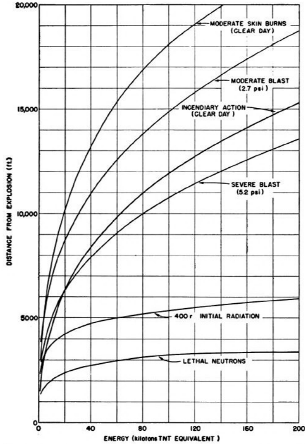
Figure 12.13. Distances from explosion at which various effects are produced as function of bomb energy.
